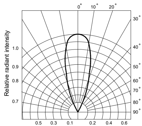
Fig.6 Radiation diagram
